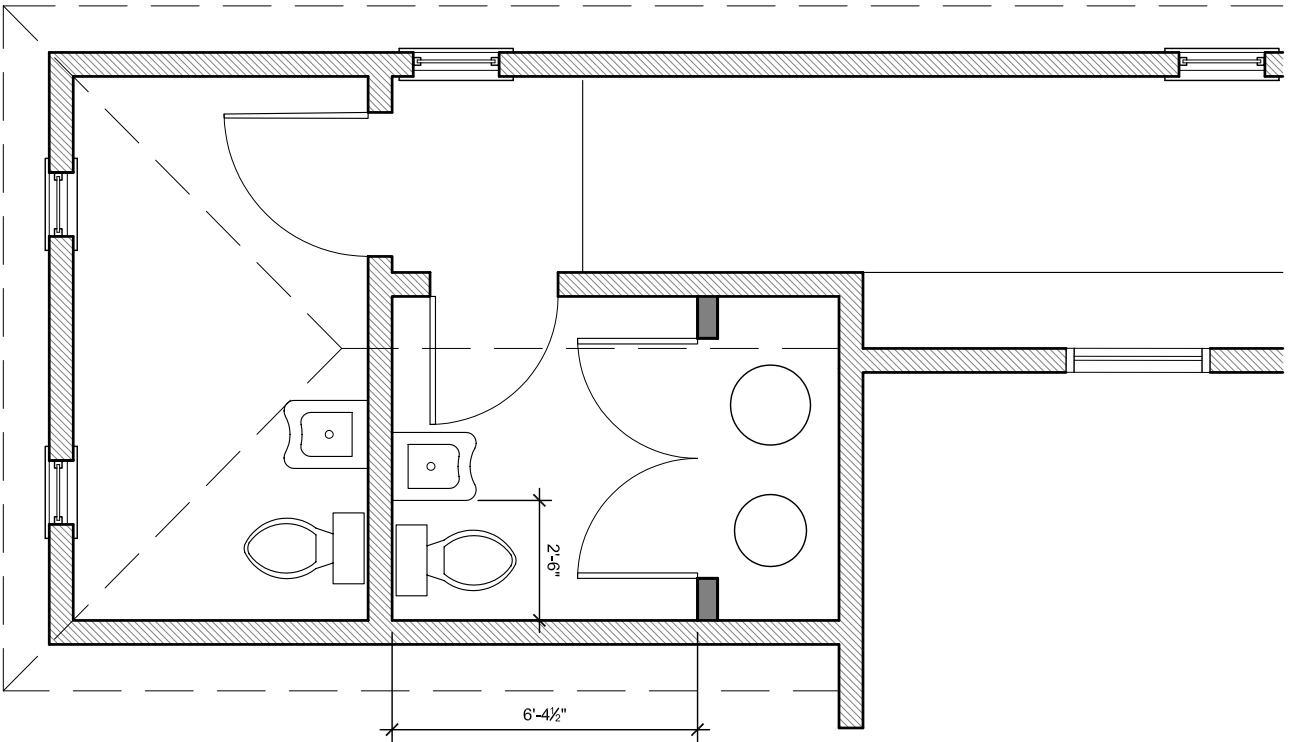
MEETING HOUSE BATHROOM PLAN 2-12-2013
