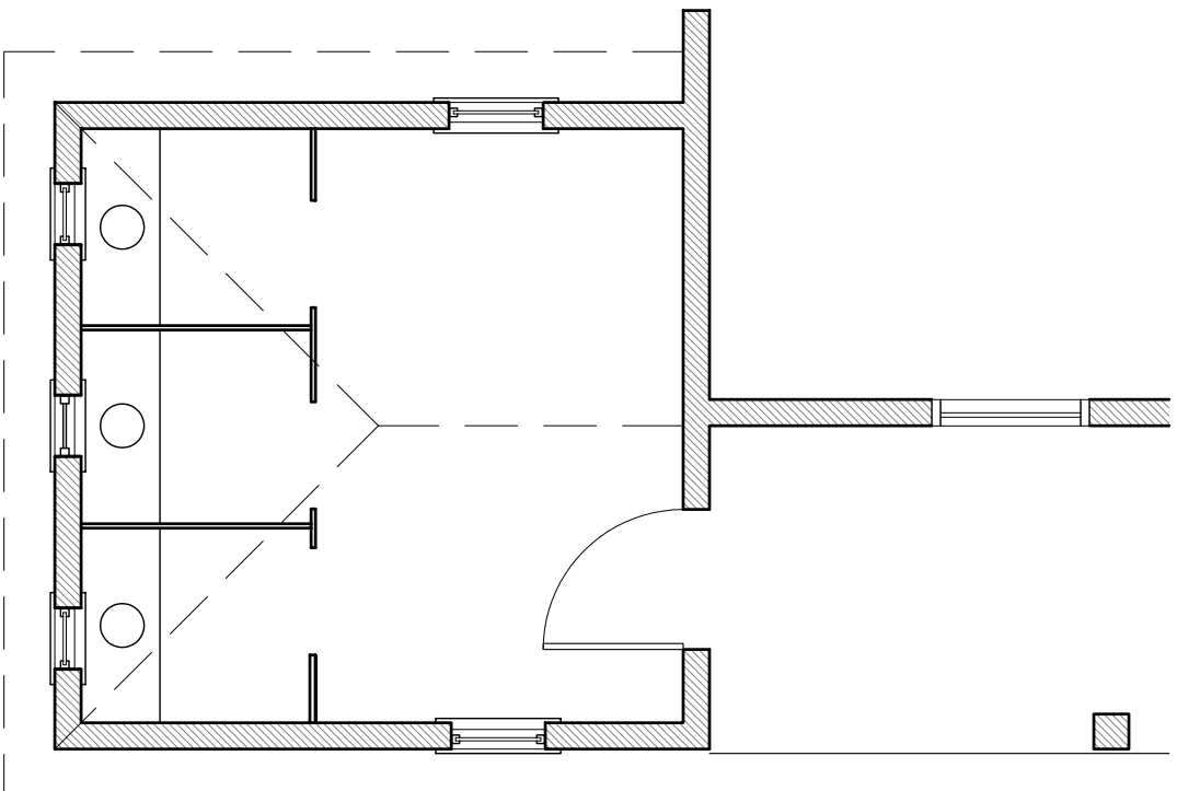
MEETING HOUSE PRIVY PLAN 2-12-2013
