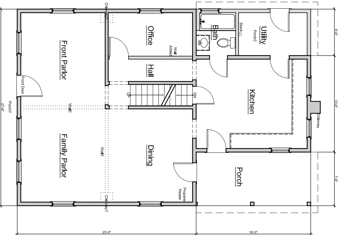
FIRST FLOOR ROUGH PLAN: 2-19-13
