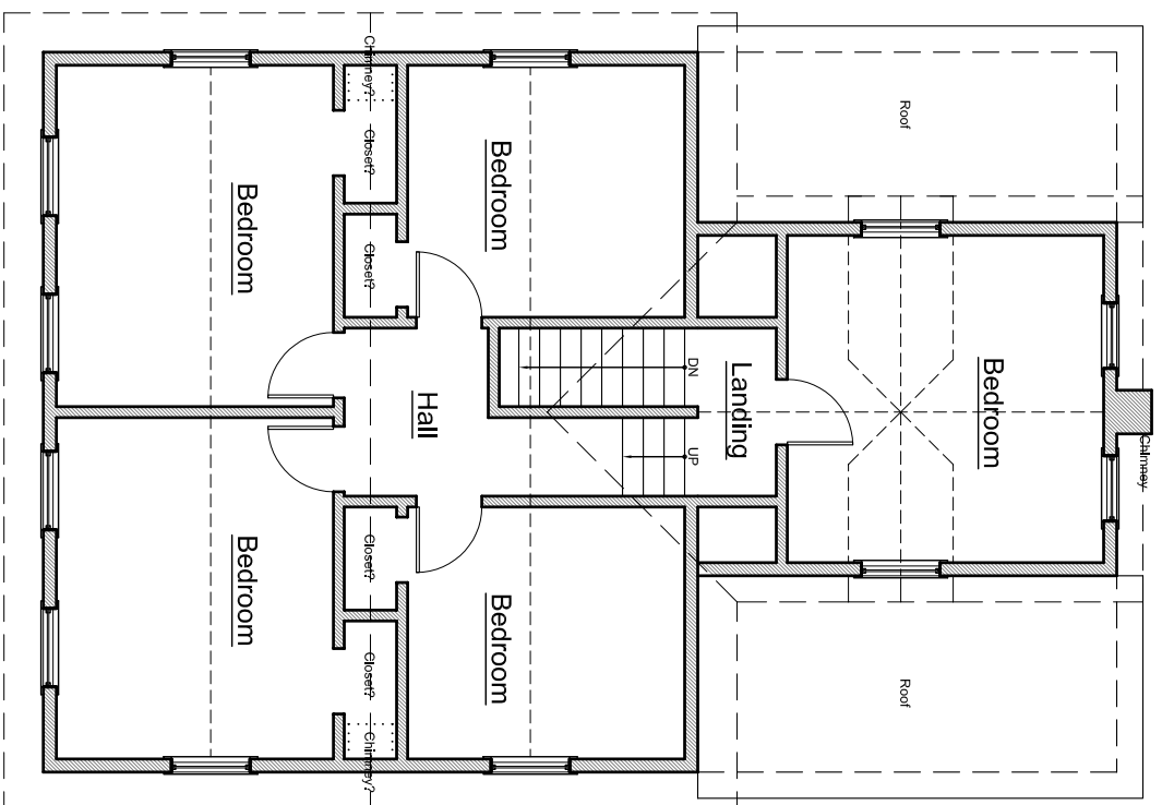
SECOND FLOOR ROUGH PLAN: 2-19-13
